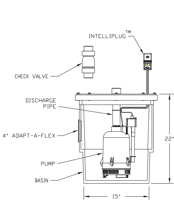
22" BASIN PACKAGE
