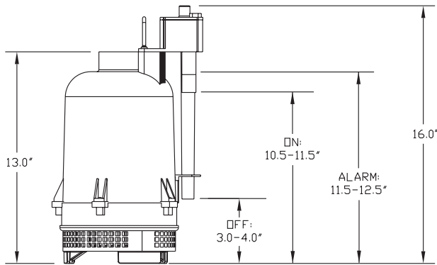
OVERALL DIMENSIONS WO/LEG KIT
