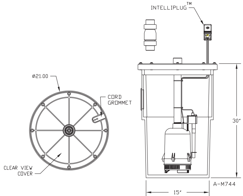
30" BASIN PACKAGE
