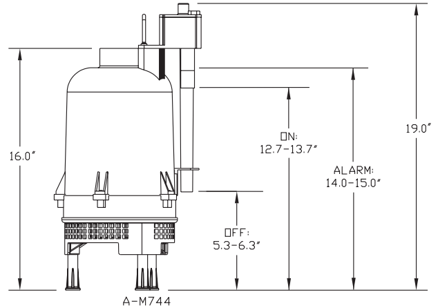
OVERALL DIMENSIONS W/LEG KIT
