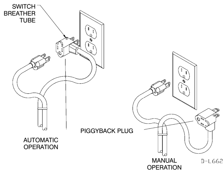
PIGGYBACK PLUG INSTALLATION FIG 1
