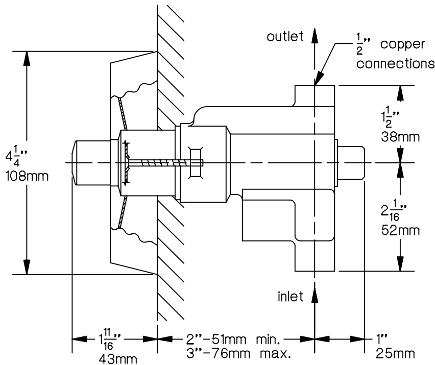
illustrated 3"-76mm from centerline of tubing to face of wall.
