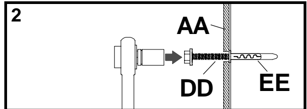
Place plate ( AA ) over anchors ( EE ) and secure with screws ( DD ).
