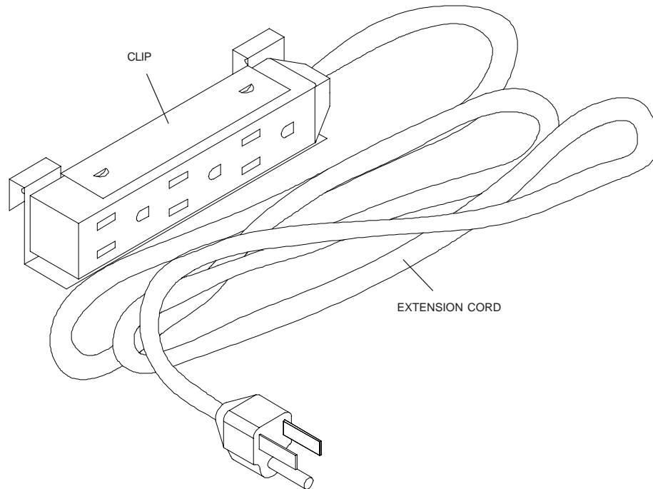
ISOMETRIC VIEW
