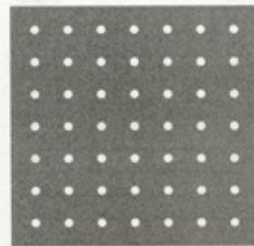
Pattern #1875 .052 in. diameter diagonal pattern 25 holes per square inch
