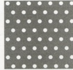
Pattern #560-85 .085 in. diameter staggered pattern 20 holes per square inch
