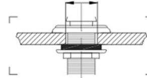
Spray Installation Hole Ø 1 1/4"
