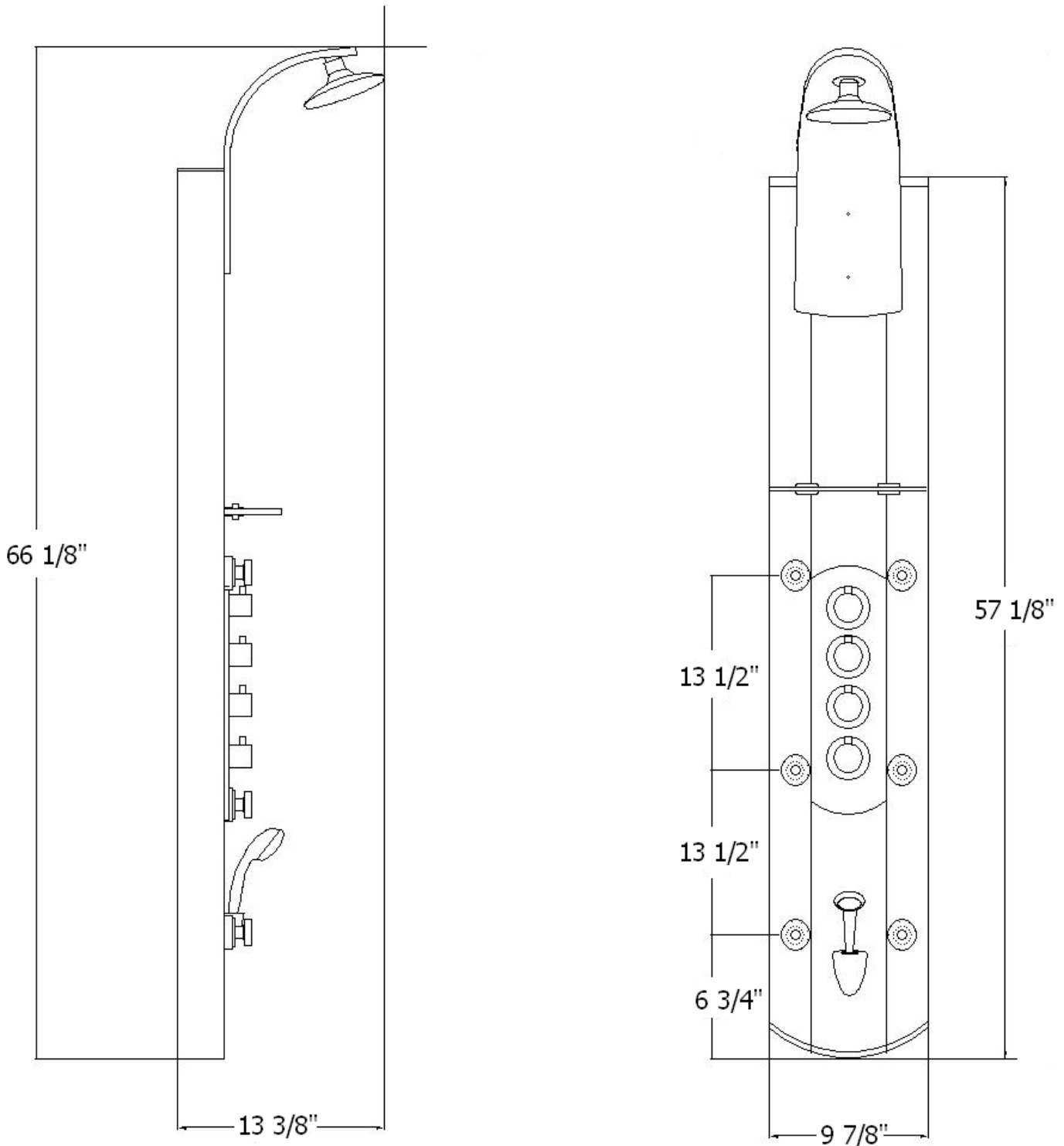
Technical Diagram
