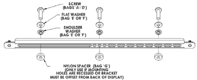
USE PROPER LENGTH, SIZE AND AMOUNT OF SCREWS/WASHERS DEPENDING ON DISPLAY MOUNTING HOLE PATTERN
