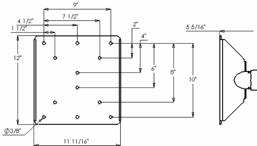
Figure 1. Base Dimensions
