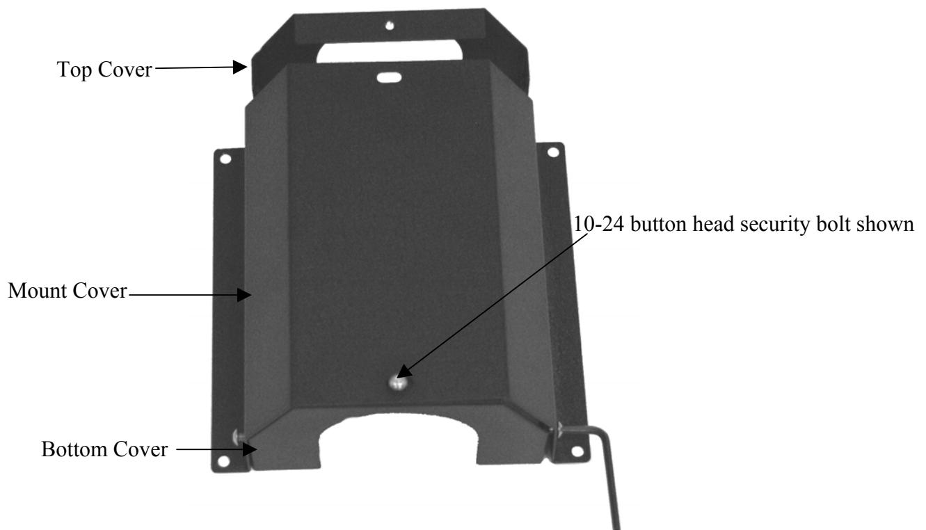
Figure 1. Attach Top and Bottom Covers
