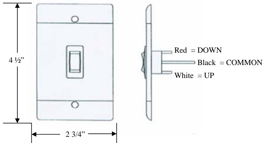
Figure 2. Dimensions and Wiring
