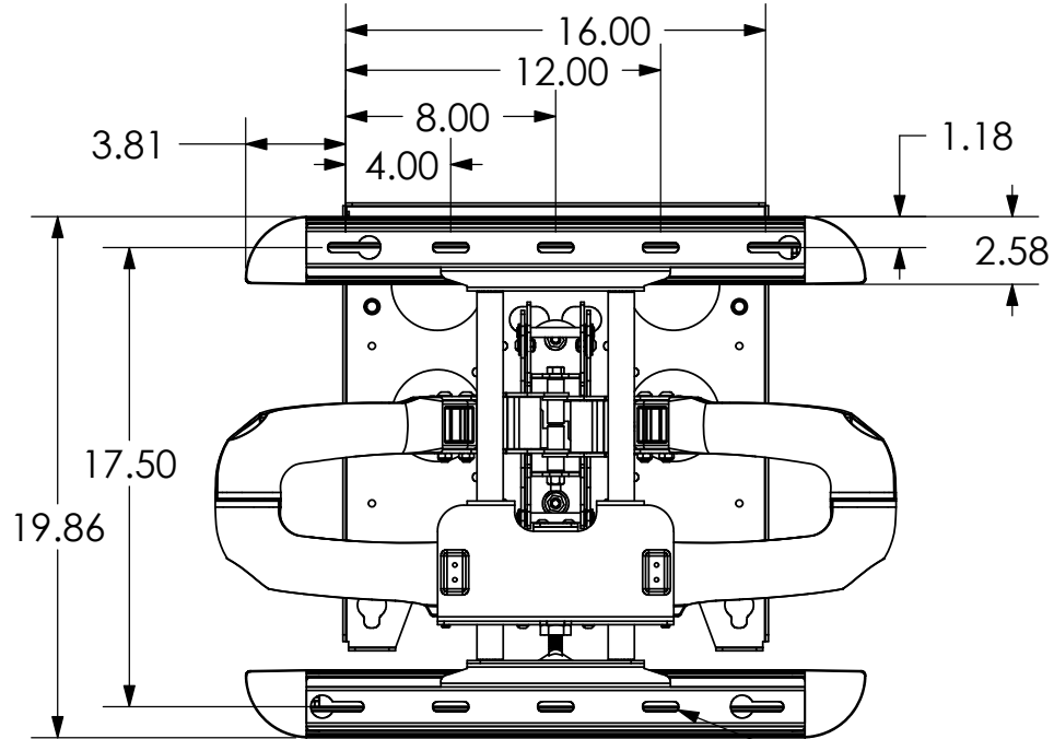
BACK VIEW
