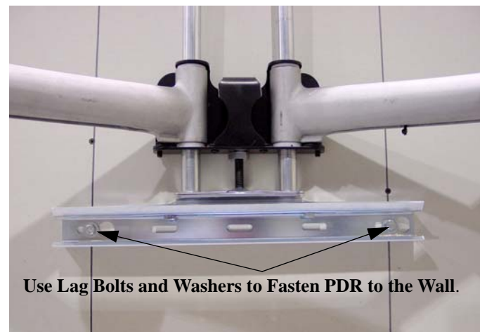
Figure 3. Mount Bottom Bracket on PDR
