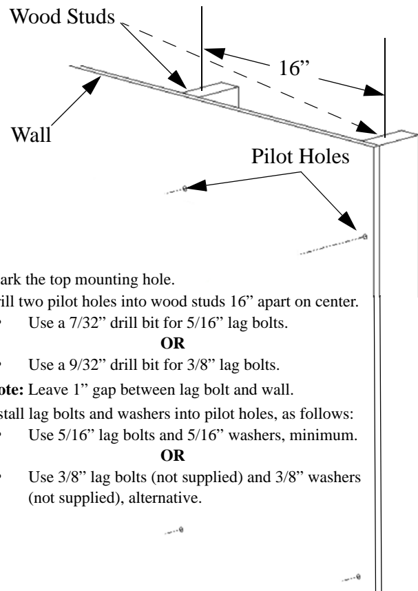
Figure 1. Two Wood Studs 16" Apart On Center
