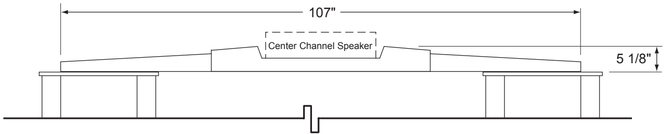
FRONT VIEW (Video Bridge for Center Channel Speaker)
