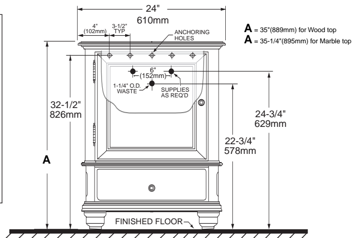
9424.200 Providence 24" Wood Vanity. Shown with Optional Ovalyn Undercounter Sink and Hampton 8" faucet.
